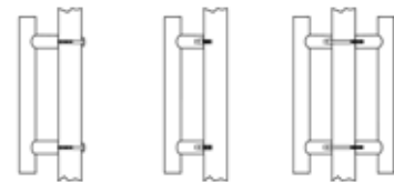
Single Thru Bolt Single Concealed Pair Back to Back
